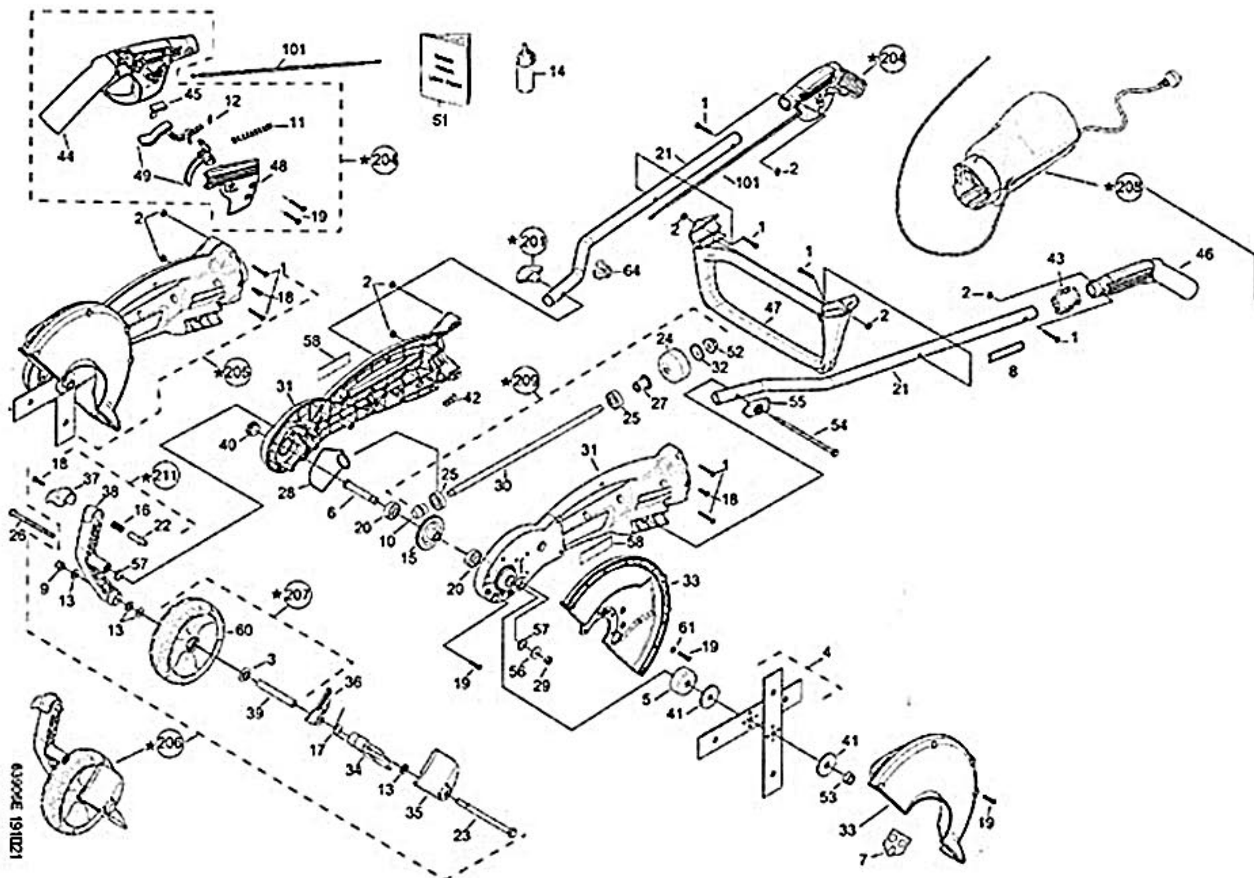
ATOM ELECTRIC EDGER MODEL 310
